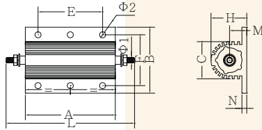
AHB75A-AHB15B TYPES & AHB25B-AHB50B TYPES
